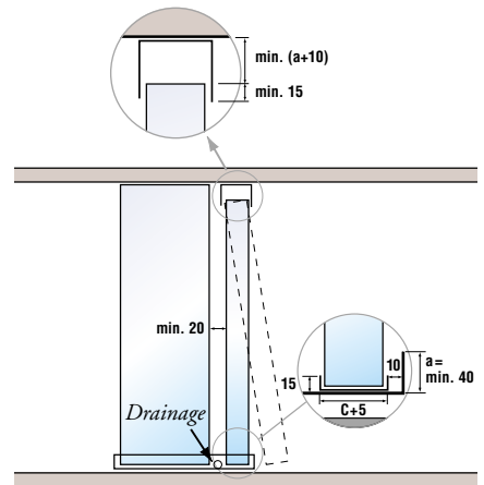
Cooling coils with level trough. Dimensions in mm.
